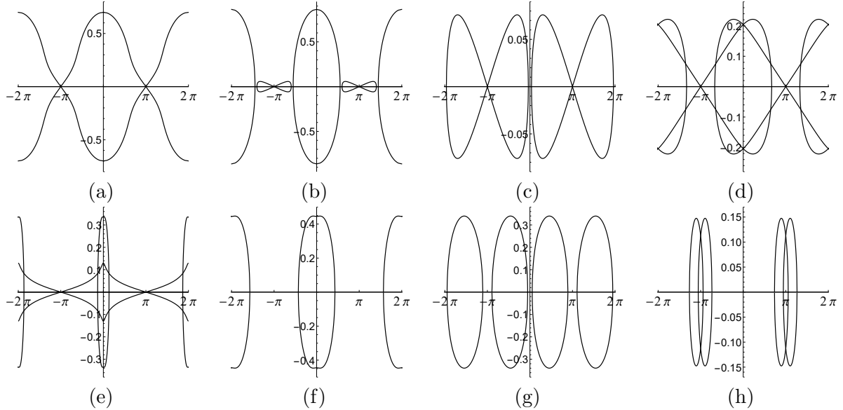
Figure 9: The real part of the spectrum \text{Re}(\lambda) (vertical axis) as a function of \mu T(k) (horizontal axis): for subluminal librational (a-b), superluminal librational (c-e), and superluminal rotational (f-h) solutions. (a) c = 0.6, E = 1.0 ; (b) c = 0.8, E = 1.5 ; (c) c = 1.5, E = 0.7 ; (d) c = 1.5, E = 1.5 ; (e) c = 1.02, E = 1.8 ; (f) c = 1.3, E = 2.9 ; (g) c = 1.4, E = 2.4 ; (h) c = 2.1, E = 6.8 .
