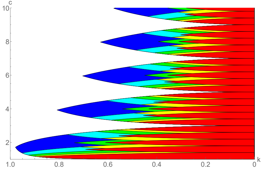
Figure 12: A plot of the superluminal rotational region of parameter space showing the spectral stability with respect to various subharmonic perturbations. Parameter space is rescaled using the elliptic modulus k = \sqrt{2/E} , to show the extent of the curves as E \rightarrow \infty . Solutions within the blue (light blue, green, yellow, red) region are stable with respect to perturbations of one (two, three, four, five) times the period respectively.
