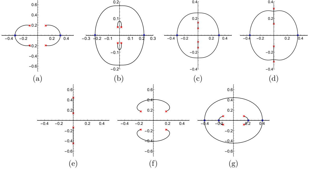
Figure 7: The Lax spectrum (black curves) for superluminal (a-d), subluminal (e-g), librational (a,b,f,g) and rotational (c,d,e) waves. (a) c = 1.5 , E = 1.5 ; (b) c = 1.02 , E = 1.8 ; (c) c = 1.1 , E = 2.2 ; (d) c = 1.4 , E = 2.4 ; (e) c = 0.6 , E = -0.75 ; (f) c = 0.6 , E = 1.0 ; (g) c = 0.8 , E = 1.5 . Red crosses signify values of \zeta for which \Omega^2(\zeta) = 0 . Blue crosses signify values of \zeta \in \mathbb{R} for which \sigma_L has a vertical tangent.
