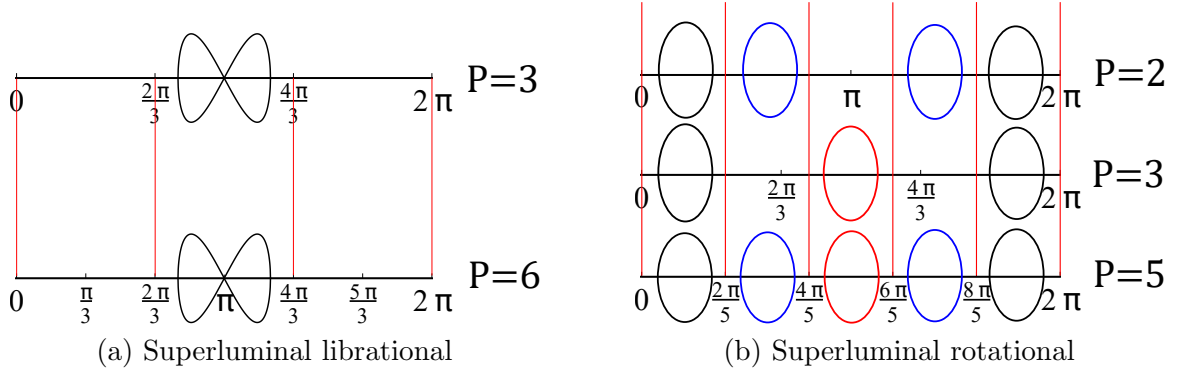
Figure 11: The real part of the spectrum \text{Re}(\lambda) (vertical axes) as a function of \mu T(k) (horizontal axes): \mu T(k) = 2m\pi/P for integers m and P corresponds to perturbations of period P times the period of the underlying solution. (a) The superluminal solution is stable with respect to perturbations of three times its period is necessarily stable with respect to perturbations of six times its period. (b) If a superluminal rotational solution is stable with respect to perturbations of five times its period, it is stable with respect to perturbations of three times its period or perturbations of two times its period. (i) If the ellipse-like curves are in (4\pi/5, 6\pi/5) they are necessarily in (2\pi/3, 4\pi/3) (red), (ii) if the ellipse-like curves are in (2\pi/5, 4\pi/5) and (6\pi/5, 8\pi/5) they are necessarily in (0, \pi) and (\pi, 2\pi) respectively (blue), (iii) if the ellipse-like curves are in (0, 2\pi/5) and (8\pi/5, 2\pi) they are necessarily in both (0, \pi) and (\pi, 2\pi) respectively as well as (0, 2\pi/3) and (2\pi/3, 4\pi/3) respectively (black).
