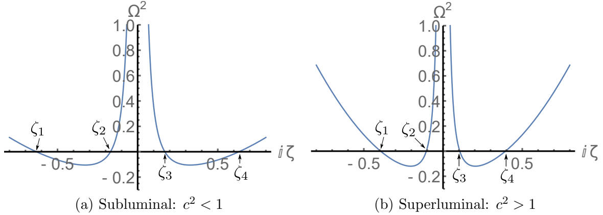
Figure 4: \Omega^2 as a function of i\zeta , \zeta \in \mathbb{R} for subluminal and superluminal rotational waves: (a) subluminal rotational: c = 0.4 and E = -1 , and (b) superluminal rotational: c = 1.4 and E = 3 .
