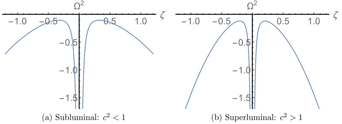
Figure 3: \Omega^2 as a function of real \zeta for subluminal and superluminal waves: (a) subluminal: c = 0.4 and E = 1 , and (b) superluminal: c = 1.4 and E = 1 .
