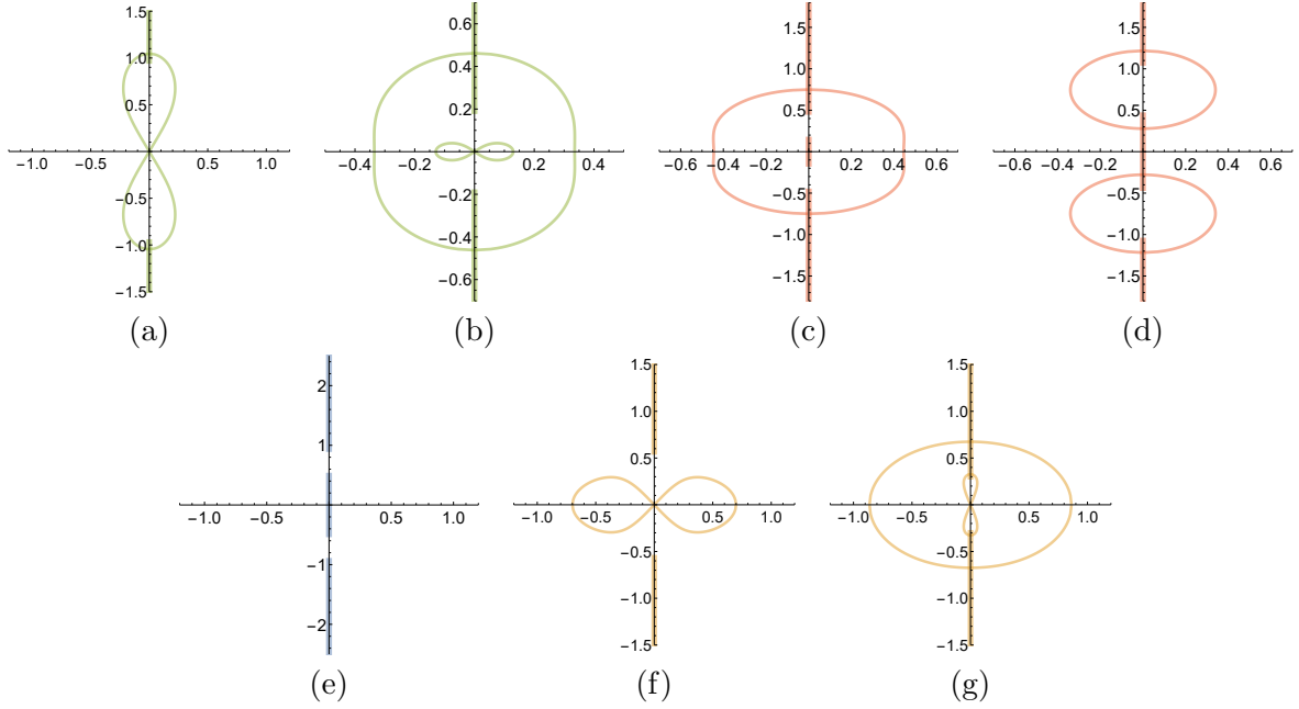
Figure 6: The stability spectrum for superluminal (a-d), subluminal (e-g), librational (a,b,f,g) and rotational (c,d,e) waves. (a) c = 1.5 , E = 1.5 ; (b) c = 1.02 , E = 1.8 ; (c) c = 1.1 , E = 2.2 ; (d) c = 1.4 , E = 2.4 ; (e) c = 0.6 , E = -0.75 ; (f) c = 0.6 , E = 1.0 ; (g) c = 0.8 , E = 1.5 ; Colors correspond to Figure 2, thickness of lines corresponds to double or quadruple covering of spectrum.
