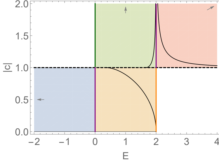
Figure 5: Parameter space with regions corresponding to different qualitative behavior in the linear stability spectrum separated by black curves. Colors correspond to solutions in Figure 1. Blue: subluminal rotational ( 0 \leq |c| < 1 , E < 0 ), orange: subluminal librational ( 0 \leq |c| < 1 , 0 < E \leq 2 ), green: superluminal librational ( |c| > 1 , 0 \leq E < 2 ), red: superluminal rotational ( 0 \leq |c| > 1 , E > 2 ).
