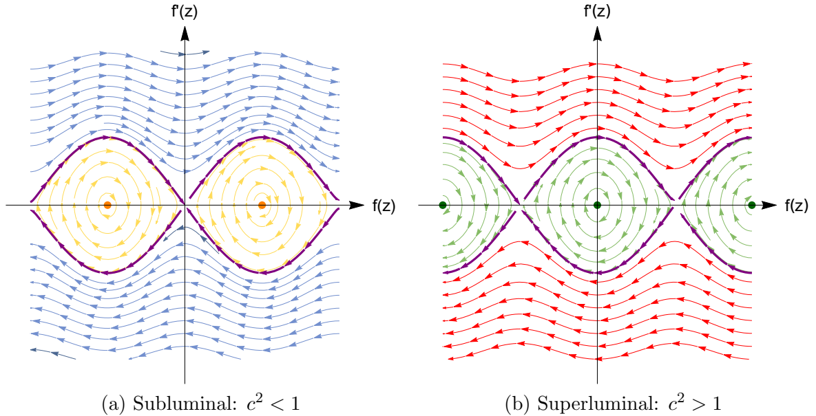
Figure 1: Phase portraits of the solutions showing both librational waves (closed orbits inside the separatrix) in yellow for (a) and green for (b) and rotational waves (orbits outside the separatrix) in blue for (a) and red for (b). The separatrix is denoted in purple.
