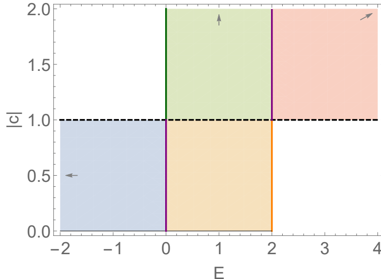
Figure 2: Subregions of Parameter space. Colors correspond to solutions in Figure 1. Blue: subluminal rotational ( 0 \leq |c| < 1, E < 0 ), orange: subluminal librational ( 0 \leq |c| < 1, 0 < E \leq 2 ), green: superluminal librational ( |c| > 1, 0 \leq E < 2 ), red: superluminal rotational ( 0 \leq |c| > 1, E > 2 ). Subregions extend to infinity in directions of arrows. Subluminal kink solutions occur for E = 0, 0 \leq |c| < 1 , and superluminal kink solutions occur for E = 2, |c| > 1 .
