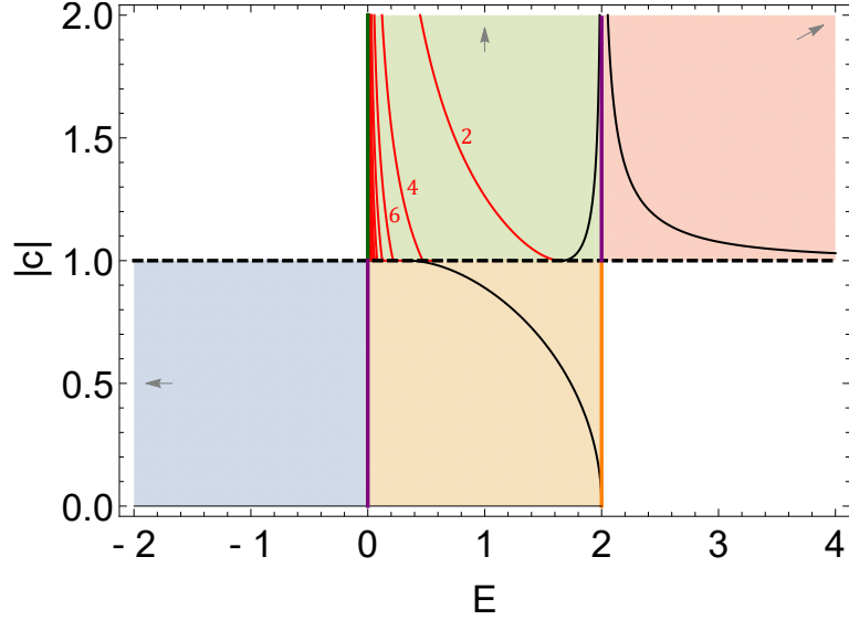
Figure 10: A plot of parameter space showing the spectral stability of superluminal librational solutions with respect to various subharmonic perturbations. Within the superluminal librational region, all solutions left of curve 2 are stable with respect to perturbations of twice the period as well as perturbations of the same period, all solutions left of curve 4 are stable with respect to perturbations of four times the period, all solutions left of curve 6 are stable with respect to perturbations of six times the period as well as perturbations of three times the period, etc.
